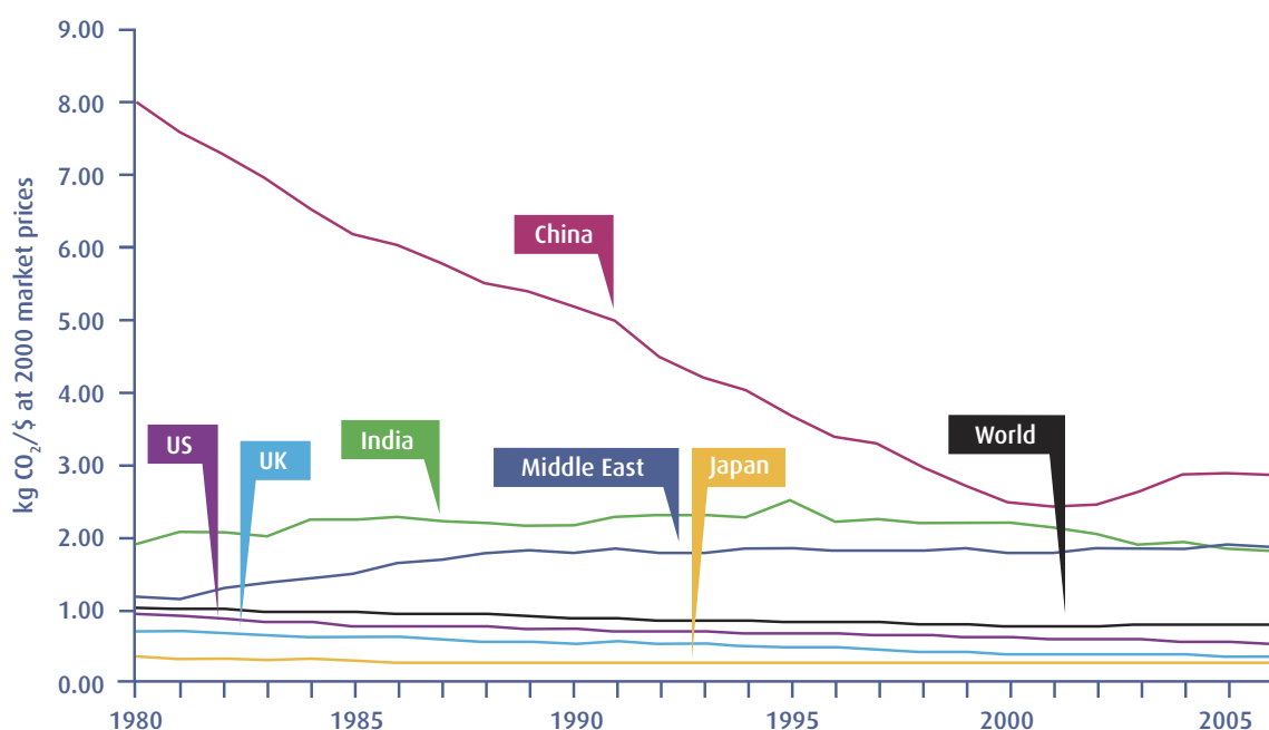
Figure 13 \text{CO}_2 intensity of GDP across nations: 1980–2006 7
